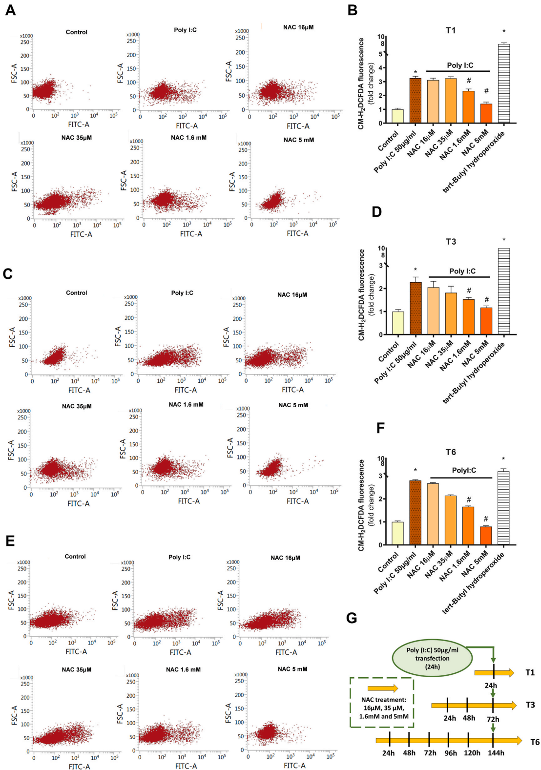
Fig. 1. NAC reduces intracellular ROS release in A549 cells. A549 cells were treated with NAC 16 μM, 35 μM, 1.6 mM and 5 mM at different timepoints and stimulated with transfected poly I:C at 50 μg/ml. Reactive oxygen species (ROS) were measured by flow cytometric analysis using the CM-H 2 DCFDA probe. (A, C, E) Representative plots for each time point are displayed: 24 h (T1), 72 h (T3) and 144 h (T6) respectively. (B, D, F) Quantification of reactive oxygen species (ROS) levels measured by the CM-H 2 DCFDA assay. Mean fluorescence of the whole living cell population
