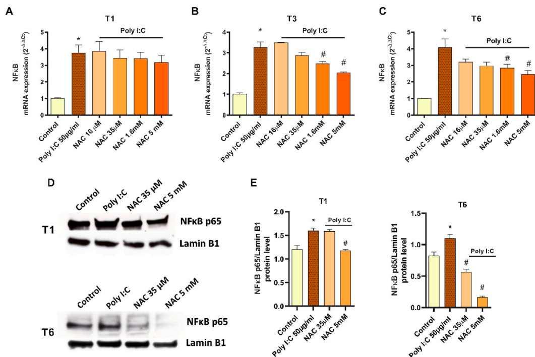
Fig. 5. NAC prevents activation of NFκB transcription factor in A549 cells. A549 cells were treated with NAC 16 μM, 35 μM, 1.6 mM and 5 mM at different time points: and stimulated with transfected Poly I:C at 50 μg/ml (A–C) NFκB mRNA levels were measured by real-time PCR at 24 h (T1), 72 h (T3) and 144 h (T6). Data are expressed as 2^{-\Delta\Delta C_t} . (D, E) NFκB p65 subunit protein levels were analyzed by Western blotting. Quantification was performed by densitometry and normalized to Lamin B1. Uncropped versions of the blots can be found in the supplemental material named “Uncropped images of the original WB”. Results are expressed as mean \pm standard error of the mean (SEM) of three independent experiments (n = 3). Statistical analysis was performed by using Kruskal-Wallis test and Dunn’s post hoc test for multiple comparisons * p < 0.05 vs. control. #p < 0.05 vs. Poly I:C. NAC: N-Acetyl-L-cysteine. POLY I:C: polyinosinic-polycytidylic.
