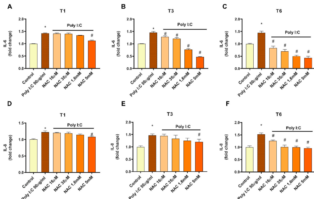
Fig. 4. NAC reduces IL-6 and IL-8 release in A549 cells. A549 cells were treated with NAC 16 \mu M, 35 \mu M, 1.6 mM and 5 mM at different time points 24 h (T1), 72 h (T3) and 144 h (T6) and stimulated with transfected Poly I:C at 50 \mu g/ml (A, B, C) IL-6, and (D, E, F) IL-8 levels were measured by ELISA. Results are expressed as mean \pm standard error of the mean (SEM) of three independent experiments ( n = 3 ). Statistical analysis was performed by using Kruskal-Wallis test and Dunn's post hoc test for multiple comparisons. * p < 0.05 vs. control. # p < 0.05 vs. Poly I:C. NAC: N-Acetyl-L-cysteine. POLY I:C: polyinosinic-polycytidylic.
