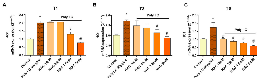
Fig. 3. NAC prevents upregulation of the antioxidant gene heme oxygenase 1 (HO1) in A549 cells. A549 cells were treated with NAC 16 \mu M, 35 \mu M, 1.6 mM and 5 mM at different timepoints and stimulated with transfected Poly I:C at 50 \mu g/ml. HO1 mRNA levels were measured by real-time PCR at (A) 24 h (T1), (B) 72 h (T3) and (C) 144 h (T6). Data are expressed as 2^{-\Delta\Delta C_t} . Results are expressed as mean \pm standard error of the mean (SEM) of three independent experiments ( n = 3 ). Statistical analysis was performed by using Kruskal-Wallis test and Dunn's post hoc test for multiple comparisons * p < 0.05 vs. control. # p < 0.05 vs. Poly I:C. NAC: N-Acetyl-L-cysteine. POLY I:C: polyinosinic-polycytidylic.
